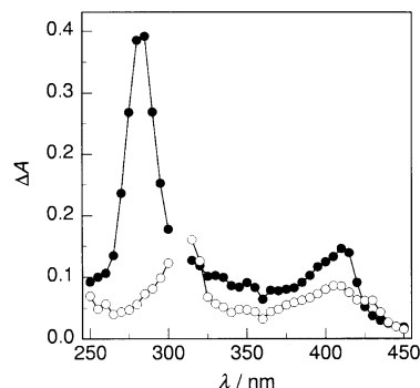
Figure 5. 308 nm laser flash photolysis of 1,4-benzoquinone (4 mM) in \text{N}_2 -saturated aqueous solution. UV/Vis spectra recorded at 100 ns ( \bullet ) and 1.4 \mu\text{s} ( \circ ) after the flash. The wavelengths close to the exciting wavelength had to be omitted.
