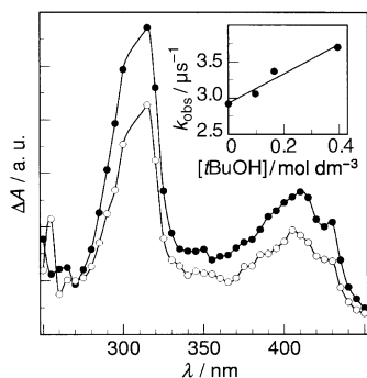
Figure 8. 308 nm laser flash photolysis UV of 1,4-benzoquinone (4 mM) in aqueous solution in the absence (●) and presence (○) of t BuOH (0.4 M). The spectra were recorded 1.4 \mu\text{s} after the flash. Inset: Observed rate constant of the decay at 285 nm of the 1,4-benzoquinone triplet as a function of the tertiary butyl alcohol concentration. The regression line yields a value of k = (1.94 \pm 0.2) \times 10^6 \text{ M}^{-1} \text{ s}^{-1} .
