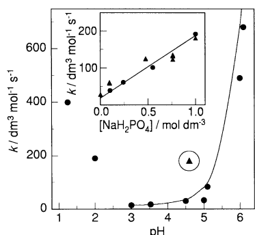
Figure 11. Observed second-order rate constant of the oxidation of 1,2,4-trihydroxybenzene by 1,4-benzoquinone as a function of pH (●) and in the presence of 1 M \text{NaH}_2\text{PO}_4 (▲). Data by stopped-flow. The solid line is calculated on the basis of the values given in the text. Inset: rate of the phosphate catalyzed oxidation as a function of the phosphate concentration at pH 4.66, laser flash photolysis LFP-LTRD (●) and stopped-flow (▲).
