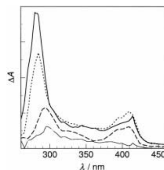
Figure 7. Global analysis of the transients. —: 1,4-benzoquinone triplet, \text{Q}^* ; .....: triplet exciplex, \text{Q}_2^* ; -----: decay product of \text{Q}_2^* , semiquinone radical \cdot\text{QH} products plus 2-hydroxy-1,4-benzoquinone, \text{QOH} ; —: decay product of \text{Q}^* , 1,2,4-trihydroxybenzene \text{Ph(OH)}_3 and/or its precursors.
